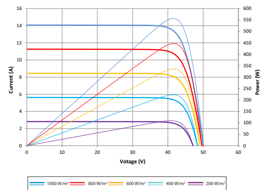
Current-Voltage & Power-Voltage Curve (555S)
